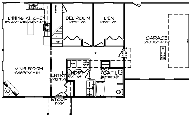
FIRST FLOOR PLAN A-4
