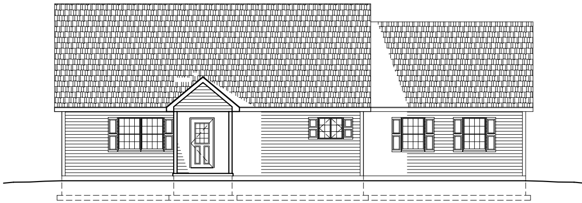
1 FRONT ELEVATION A-1
