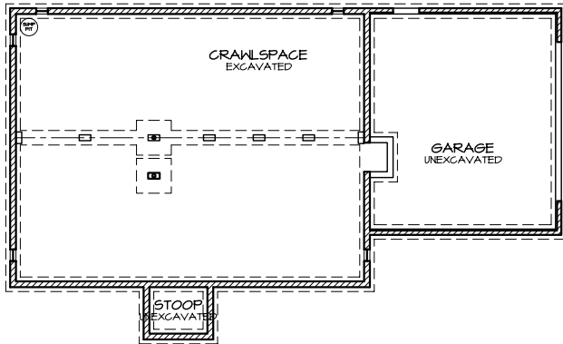
FOUNDATION PLAN A-3
