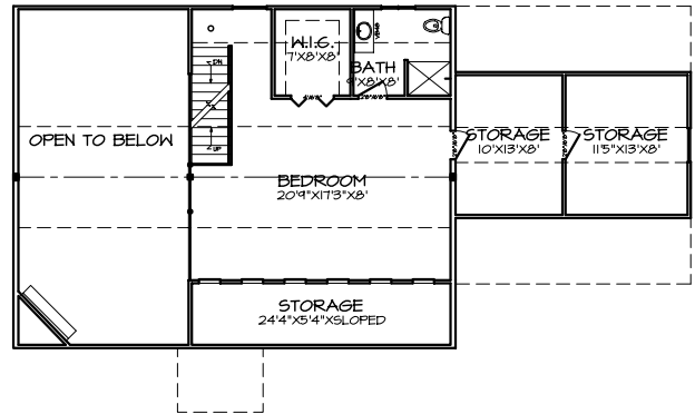
SECOND FLOOR PLAN A-5
